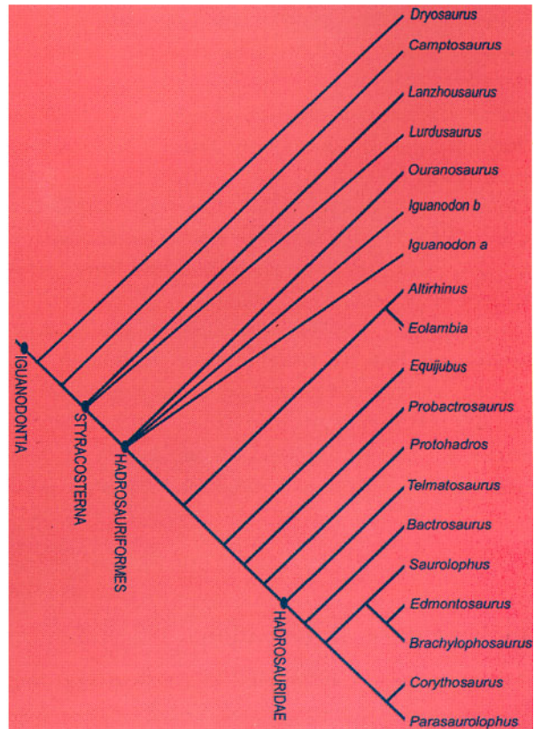
Fig.4 Phylogenetic relationship of Lanzhousaurus magnidens gen. et sp. nov. to other iguanodontian dinosaurs. The topology is based on the strict consensus of six equally parsimonious and shortest trees from a PAUP branch-and-bound search for 79 characters of 19 comparative taxa, with all multi-state characters unordered. (CI : 0.68 ; RI : 0.86)
